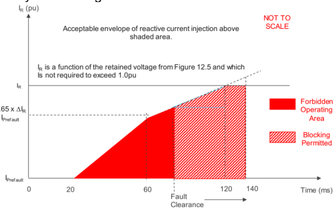
Figure 12.6(a) Chart showing area of reactive current injections for voltage depressions of \leq 140 ms duration
