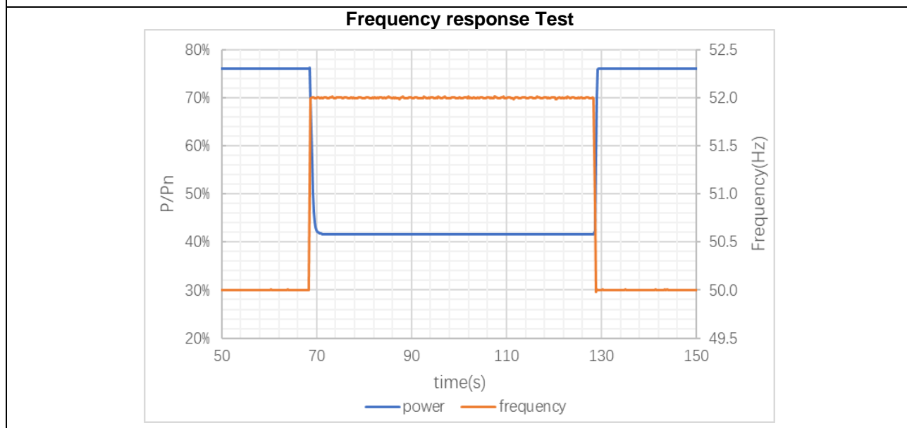
Figure B.6.1(i): LFSM-O step response test – frequency injection
