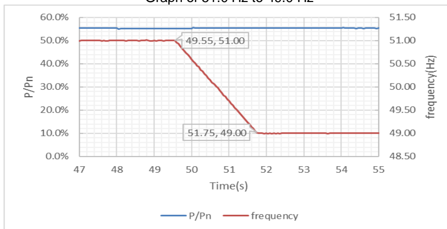
Graph of 51.0 Hz to 49.0 Hz
