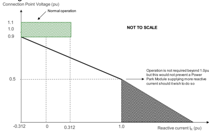
Figure 12.5 – locus of magnitude of injected Reactive Current
