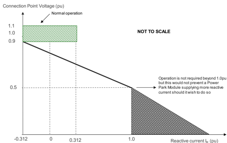
Figure 12.6 – locus of magnitude of injected Reactive Current
