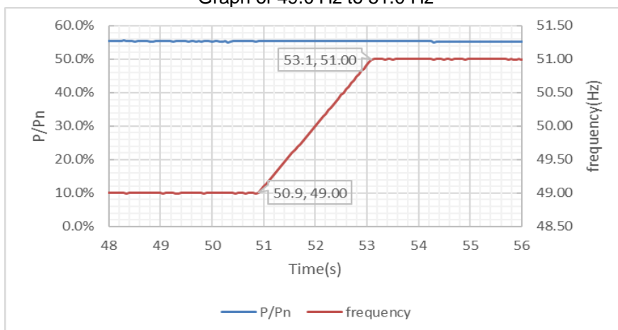
Graph of 49.0 Hz to 51.0 Hz
